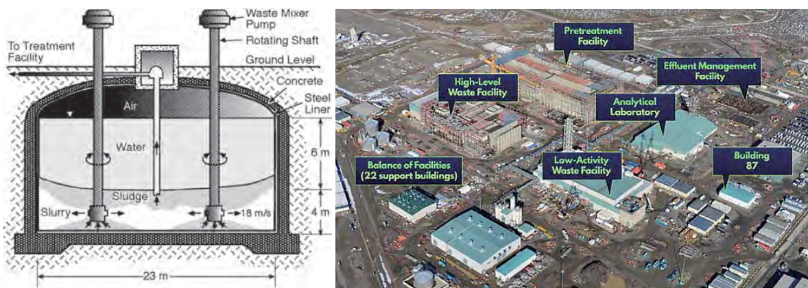
Figure 24. Waste retrieval from double shell tanks and Waste Treatment and Immobilization Plant under construction
